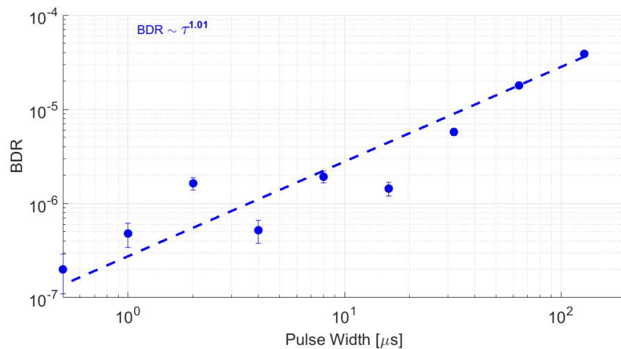
Fig. 1. BDR vs pulse width dependency for soft copper electrodes for the pulse width 500 ns – 128 \mu\text{s} . The applied voltage is 4500 V (75 MV/m).
